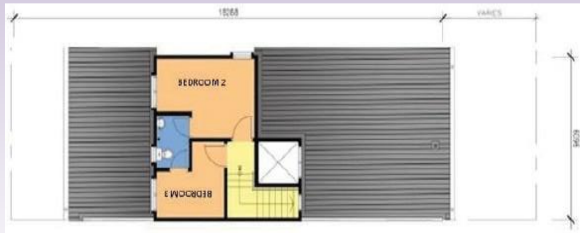
1st Floor
